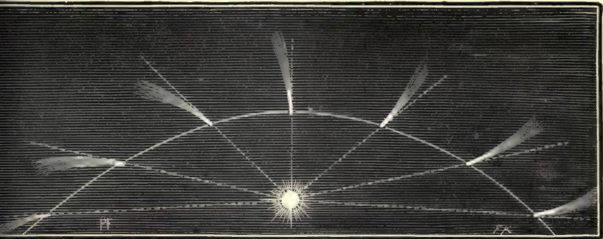
DIAGRAM ILLUSTRATING CHANGES IN THE DIRECTIONS OF THE TAILS OF COMETS.
